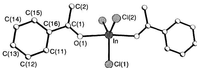
Fig. 4 The molecule [\text{InCl}_3(\text{PhCOMe})_2] , with the In-Cl(1) bond providing the C_2 axis. The atoms of the ligand molecules are almost coplanar with InCl(1)O(1)O(1'). A spreading of the O(1)-In-O(1') angle arising from \text{CH}_3 \cdots \text{Cl}(2)/\text{Cl}(2') repulsions is apparent
